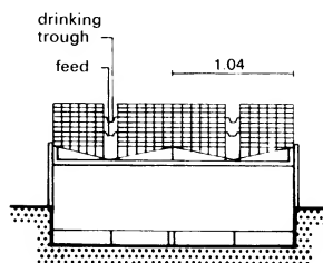
⑨ Flat deck cages
